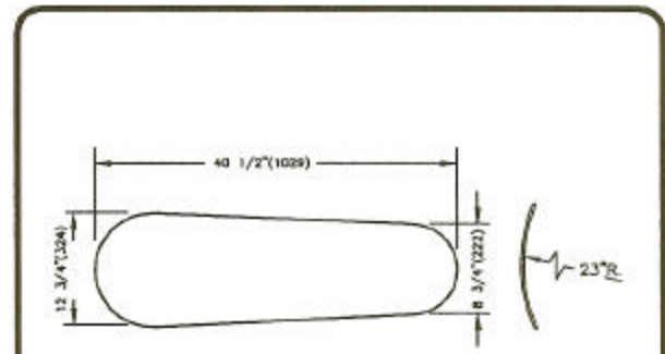
Buck Dimensions
